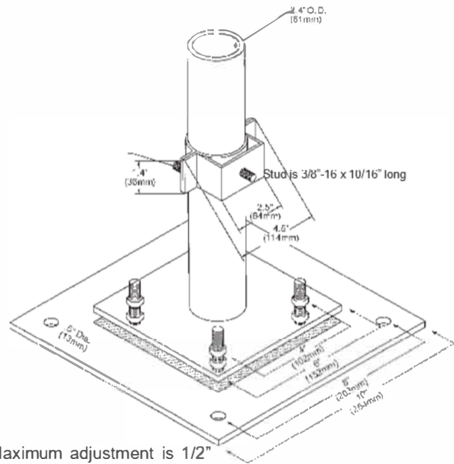
Figure 13: Pedestal Dimensions
