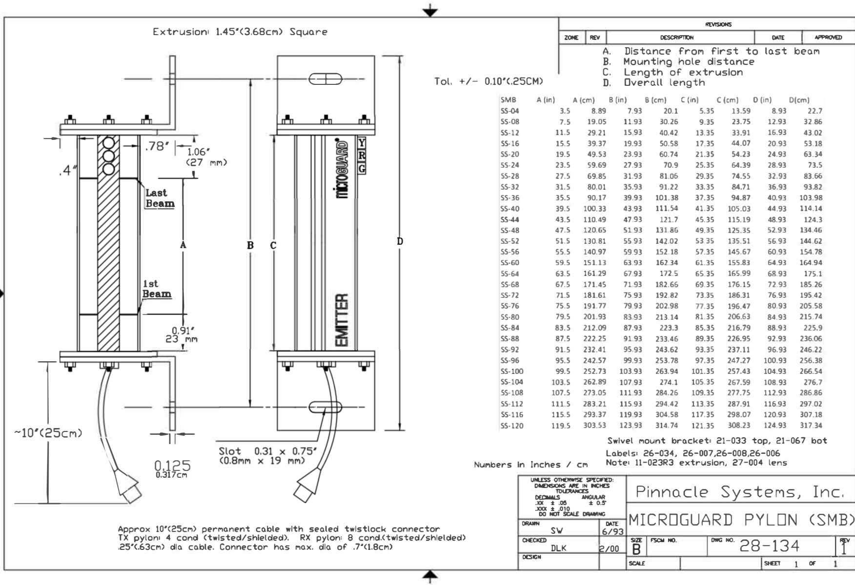
Figure 8: Swivel Bracket Dimensions, pylon dimensions (by model), and additional cable information
