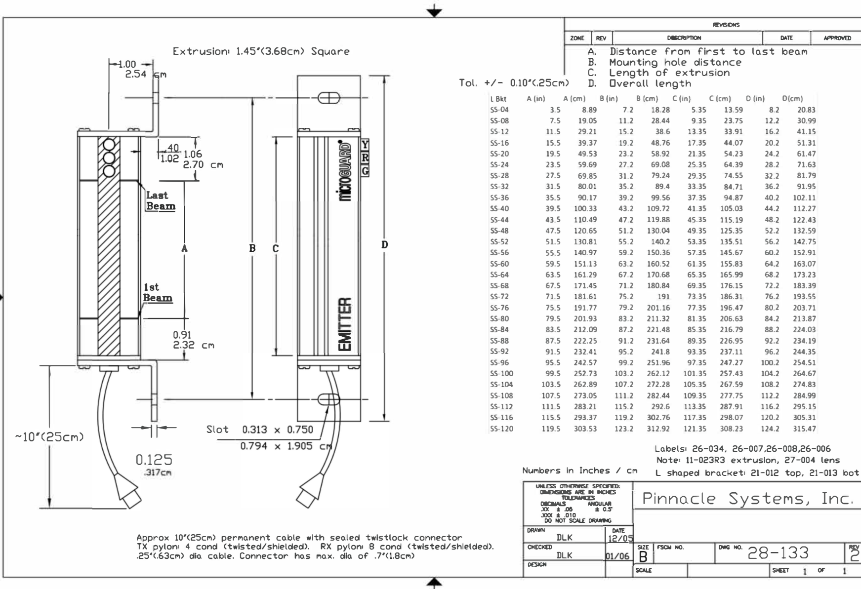
Figure 10: Fixed Bracket Dimensions, pylon dimensions (by model), and additional cable information
